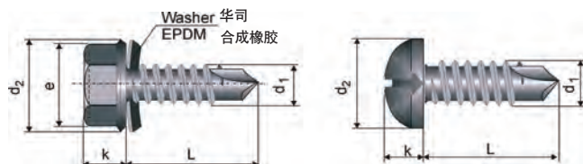
Fig.4 Self-Drilling Tek Screws 图四 Tek 钻尾螺丝
